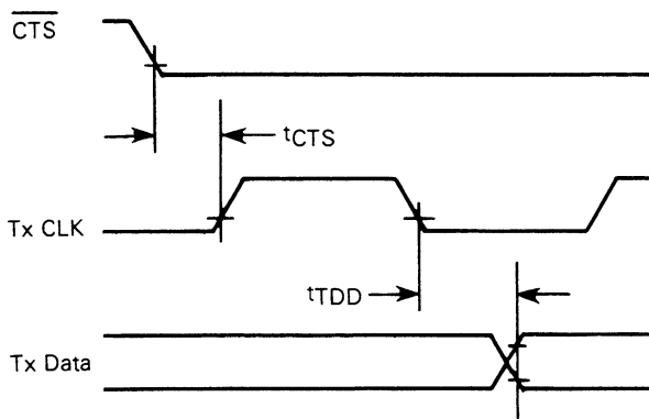
FIGURE 6 — CLEAR-TO-SEND SETUP TIME
