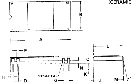
CASE 716-06 (CERAMIC)
