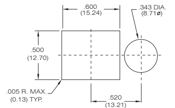
PANEL MOUNTING
