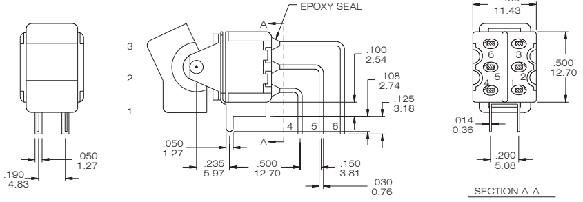
R8011L - R11-2-Q Please see page B12 to know more about R812L (3-way Switches)
