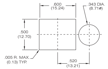
PANEL MOUNTING
