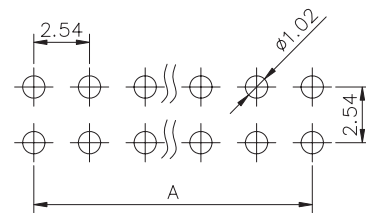
RECOMMEND P. C. BOARD LAYOUT PCB TOLERANCE: ±0.05 (TOP VIEW)
